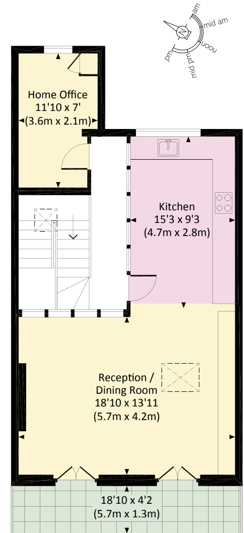
THIRD FLOOR
